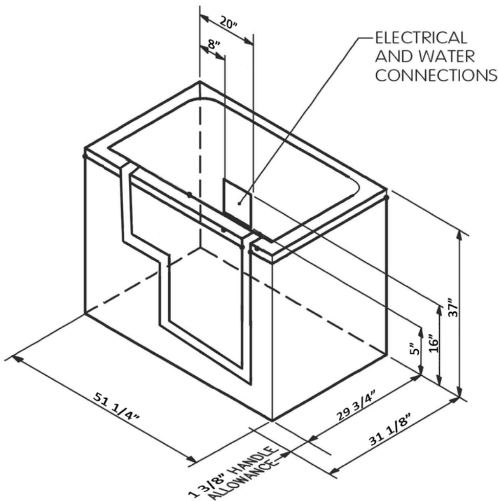
Right-Hand Rough-In
