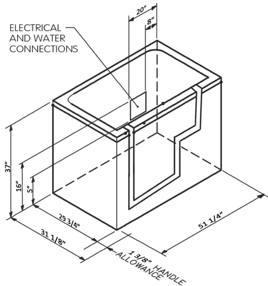
Left-Hand Rough-In
